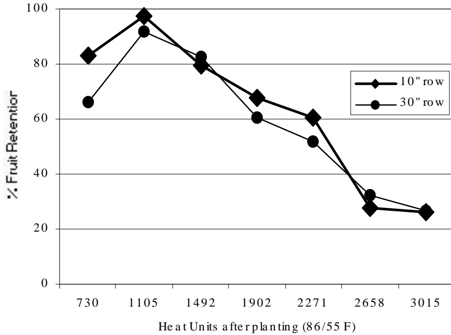
Figure 1. Cotton fruit retention as a function of heat units accumulated after planting for 10" and 30" row spacings.
