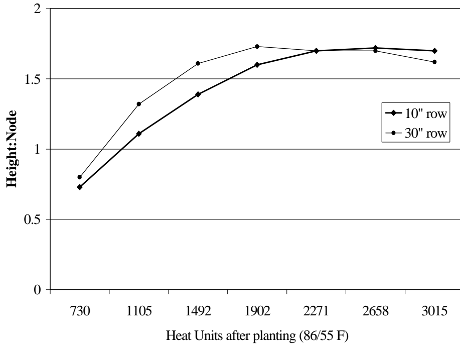
Figure 2. Cotton height:node ratio as a function of heat units accumulated after planting for 10" and 30" row spacings.
