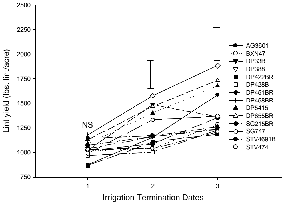
Figure 12. Lint yield as affected by irrigation termination dates for each variety, MAC, 2002.
