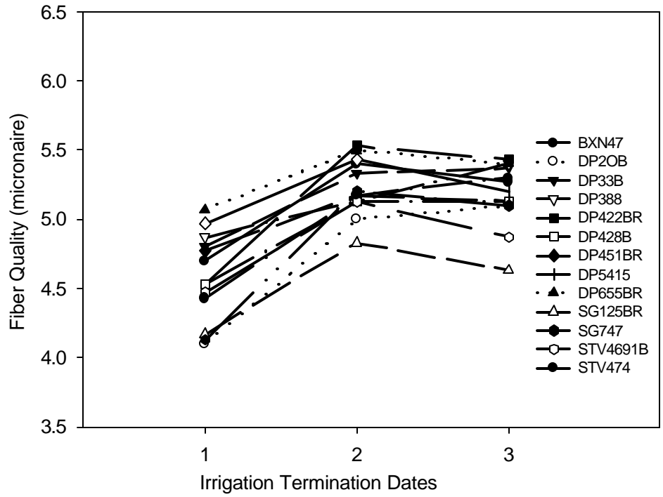
Figure 2. Micronaire values as affected by irrigation termination date for each variety, MAC, 2000.
