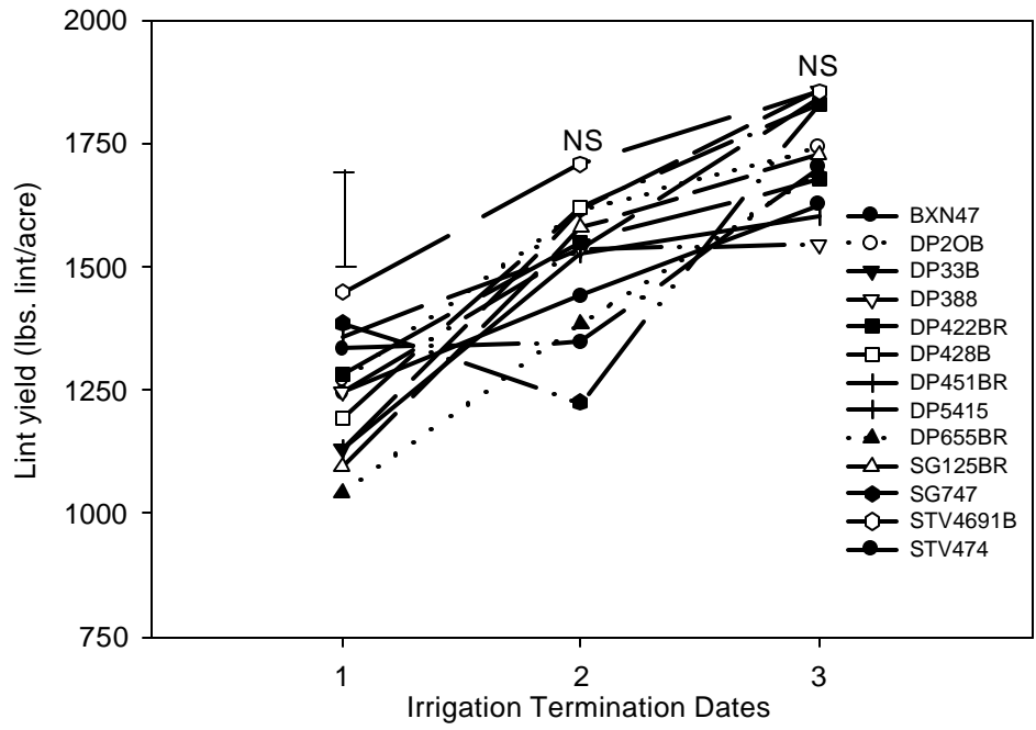
Figure 4. Lint yield as affected by irrigation Termination Dates for each variety, MAC, 2000.
