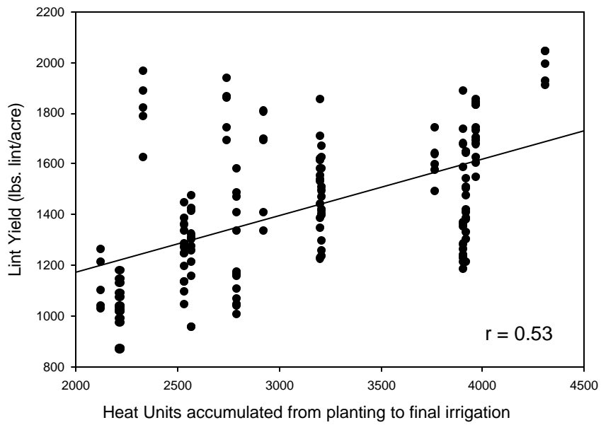
Figure 27. Relationship between lint yield and heat units accumulated from planting (PD) to final irrigation (IT), MAC and YVAC, 2000-2002.
