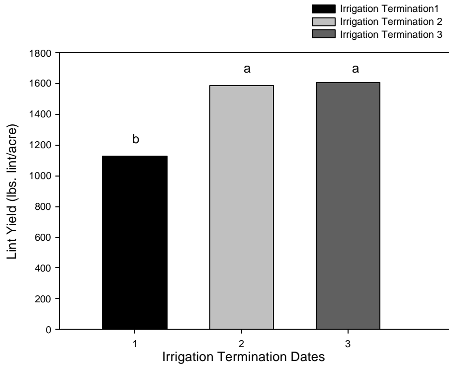
Figure 21. Mean lint yield as affected by irrigation termination dates for all varieties, YVAC, 2002.
