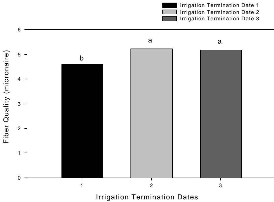
Figure 3. Mean micronaire values as affected by irrigation termination dates for all varieties, MAC, 2000.
