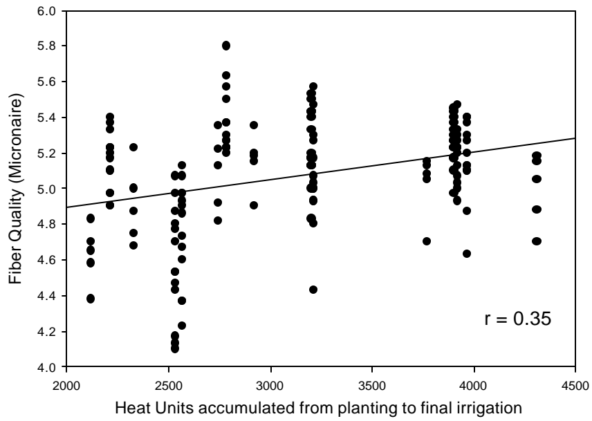
Figure 26. Relationship between fiber micronaire and heat units accumulated from planting (PD) to final irrigation (IT), MAC and YVAC, 2000-2002.
