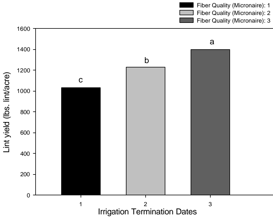
Figure 13. Mean lint yield as affected by irrigation termination dates for all varieties, MAC, 2002.
