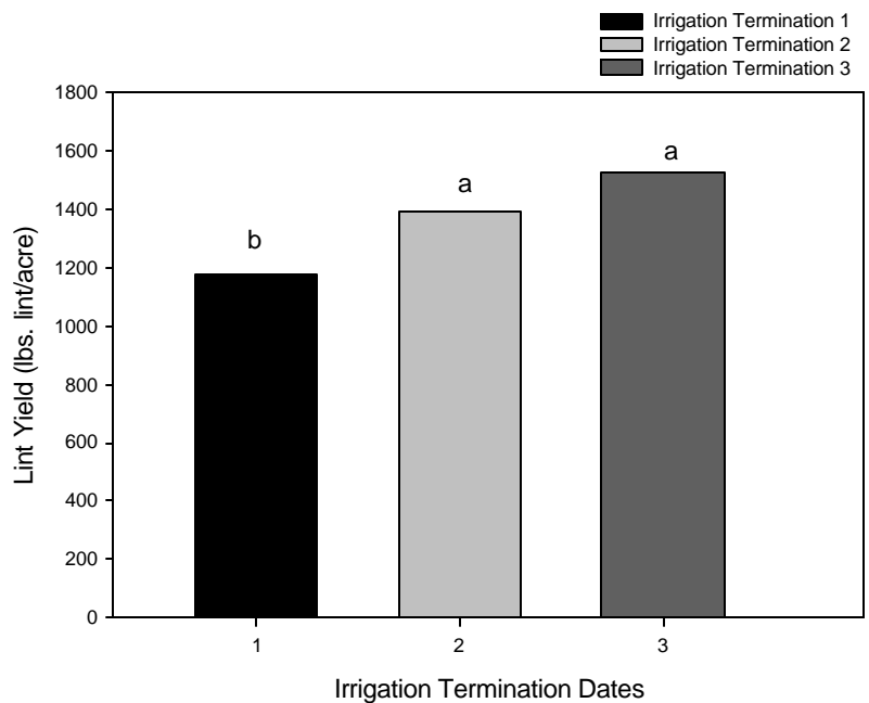
Figure 23. Grand mean of lint yields as affected irrigation termination dates for all varieties, MAC, 2000-2002.
