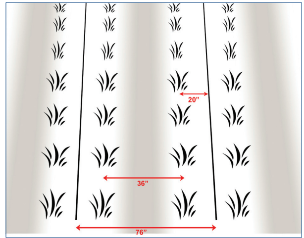
Figure 2. Example of a field where the drip tape is evenly spaced (76 inches apart) but the rows are not.
