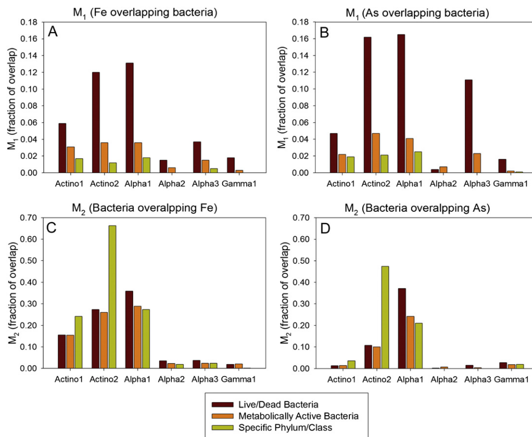
Fig. 4. Manders coefficients ( M_1 and M_2 ) for overlap of Fe and As with live/dead bacteria, metabolically active bacteria, and specific phyla/classes. (A) M_1 , representing the fraction of Fe overlapping with bacteria, (B) M_1 , representing fraction of As overlapping with bacteria, (C) M_2 , representing the fraction of bacteria overlapping with Fe, (D) M_2 , representing fraction of bacteria overlapping with As. Note the difference in scales between A and B ( M_1 values) and C and D ( M_2 values).
