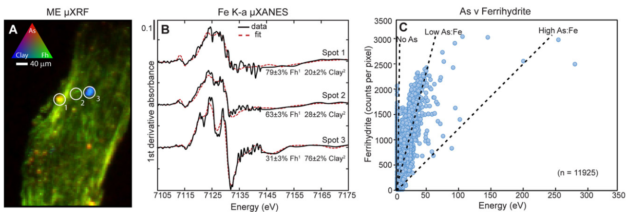
Fig. 3. B. dactyloides root. (A) Multiple-energy microfocused X-ray fluorescence (ME μ-XRF) image showing As (in red) associated with a ferrihydrite like ferric hydroxide phase (in green) and areas of Fe rich clay, fit as chlorite (in blue, e.g. spot 3) that are not associated with As. The ferrihydrite-like plaque coats the root. The color intensity scale for As, Fe-rich clay (chlorite), and ferrihydrite are 0–50, 0–150, and 0–2500 counts respectively to highlight the As relative to the more abundant ferrous Fe. (B) Microfocused (2 μm spot) XANES of select spots on the root were fit to Fe minerals, 1Fh = ferrihydrite (synthetic, Root et al., 2009) and 2Clay = chlorite clay (CCA-2, Clay Minerals Society Source Clays Repository, spectra from O'Day et al., 2004), binary fit with standard deviation shown above in panel. (C) Per pixel correlation of As to ferrihydrite, showing regions of high (e.g. spot 1), low (e.g. spot 2) and no As associated with the ferric mineral plaque. Dashed lines in C) point out that some pixels ( n = 11,925 pixels) contain no As, while many pixels have both As and ferrihydrite; at low (1:60) and high (1:12) As:Fe ratios.
